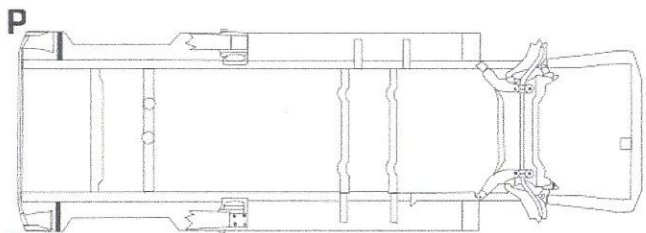
UNDERBODY VIEW
